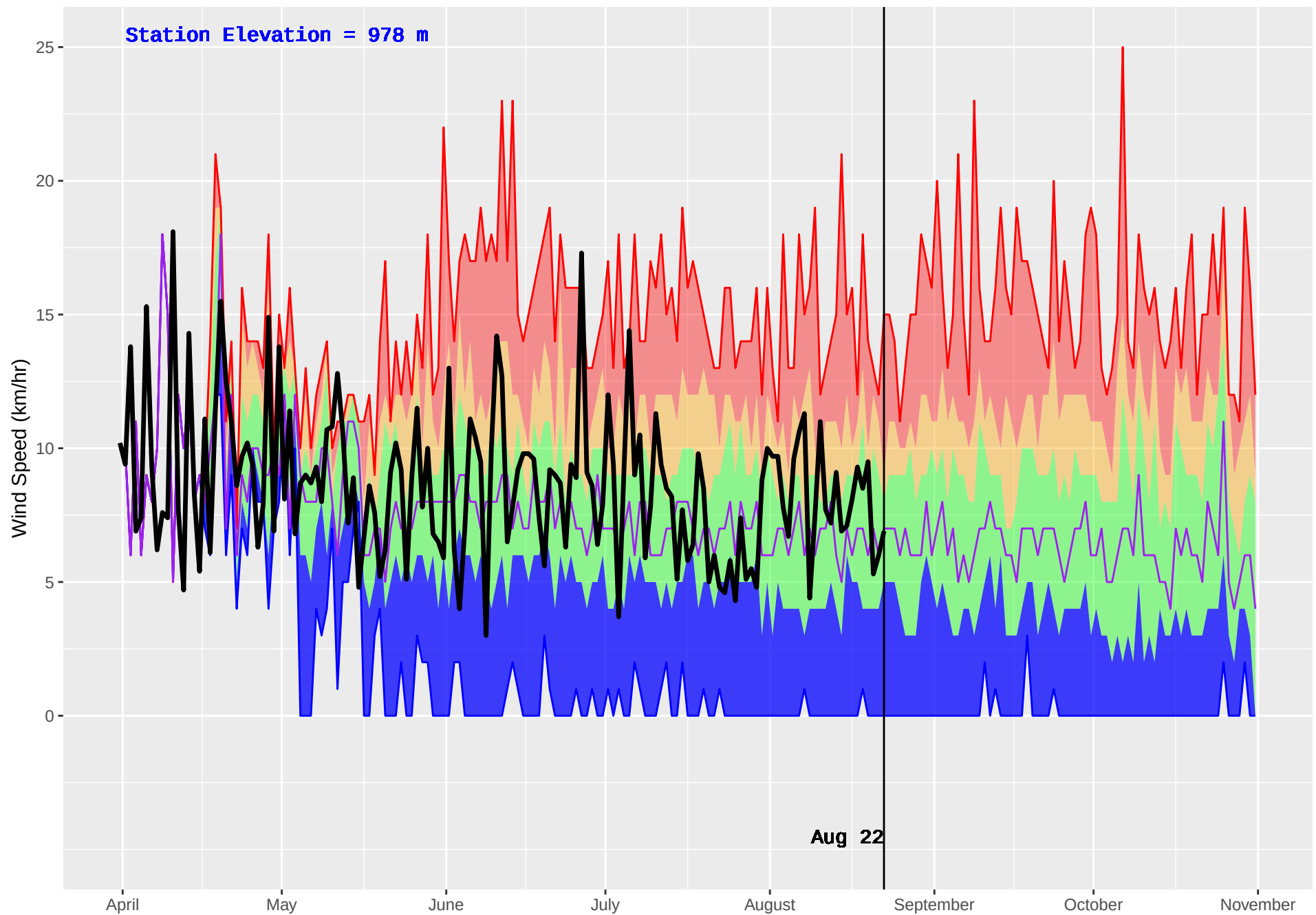
NILKITKWA (172) : Historical (1986–2016) and Current (2018) Daily Wind Speed
