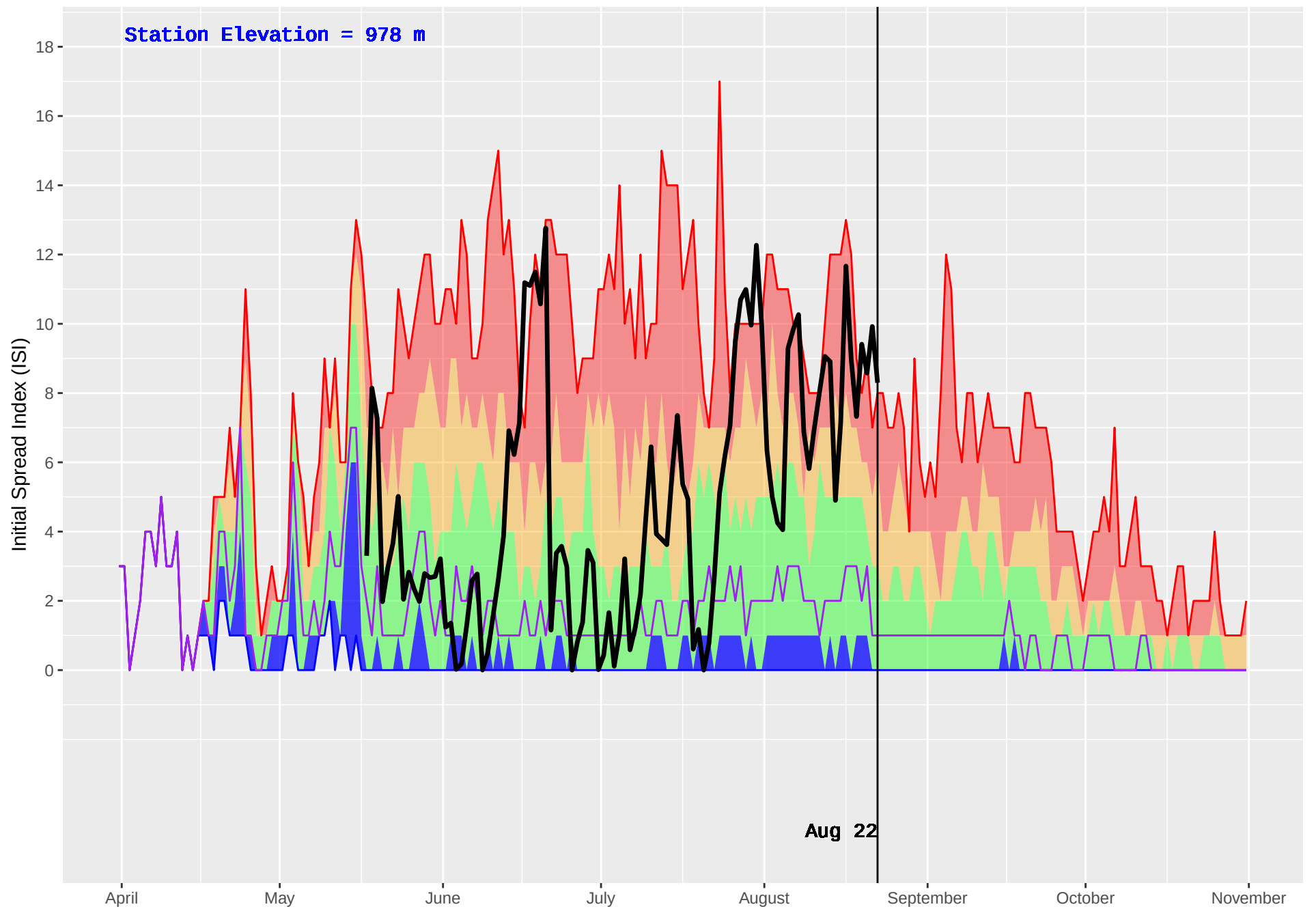
NILKITKWA (172) : Historical (1986–2016) and Current (2018) Daily Initial Spread Index (ISI)
