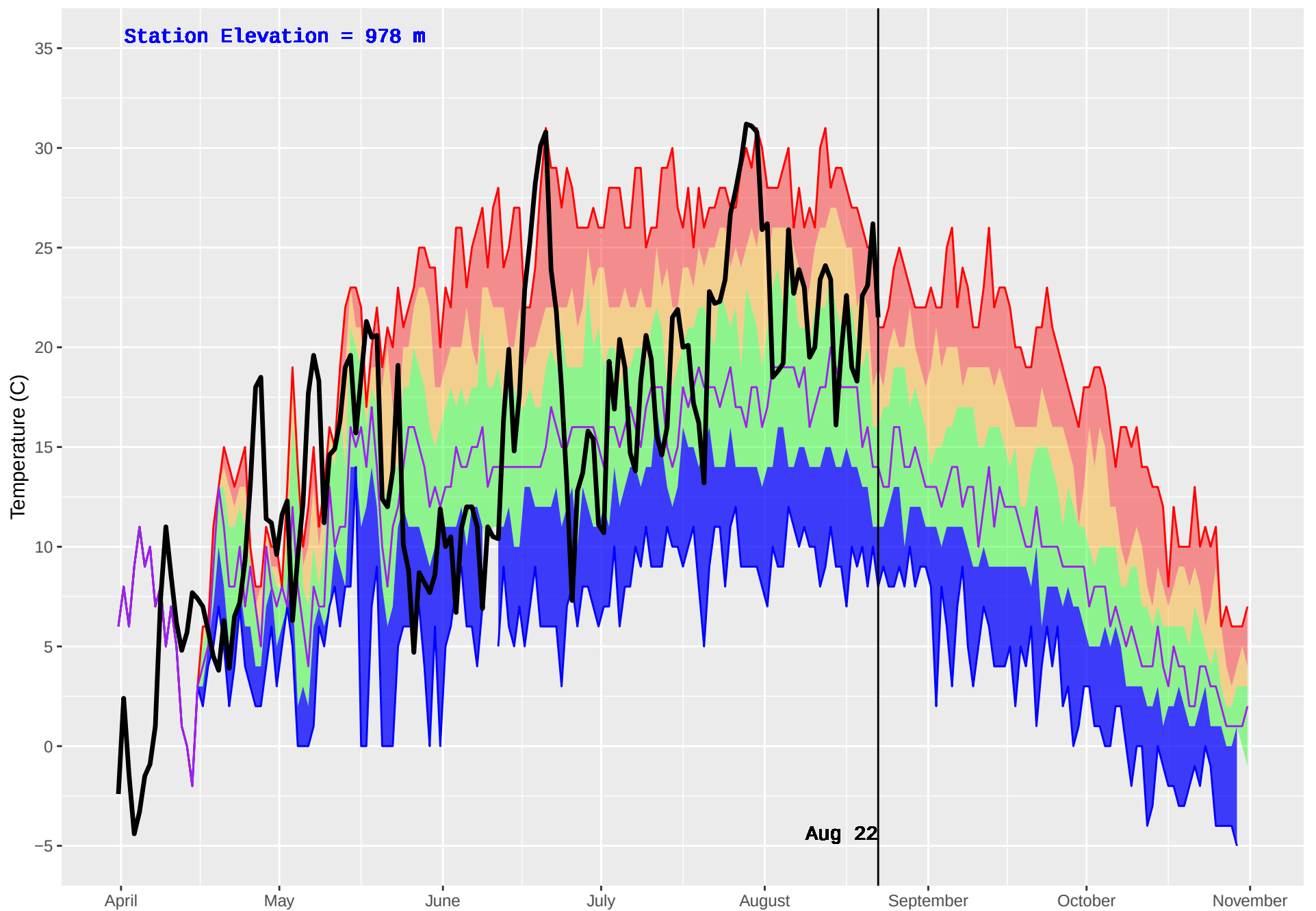
NILKITKWA (172) : Historical (1986–2016) and Current (2018) Daily Temperature
