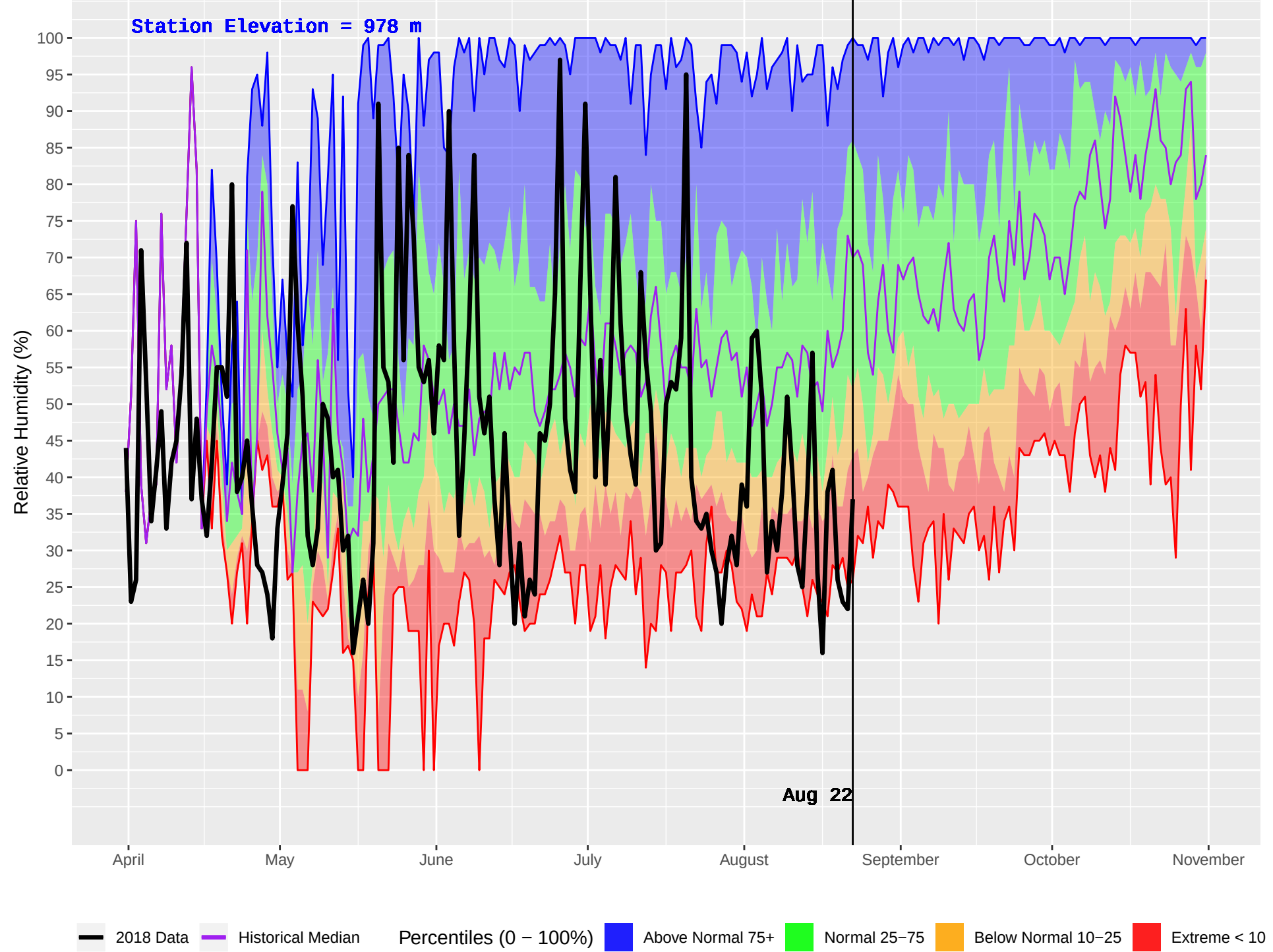
NILKITKWA (172) : Historical (1986–2016) and Current (2018) Daily Relative Humidity
