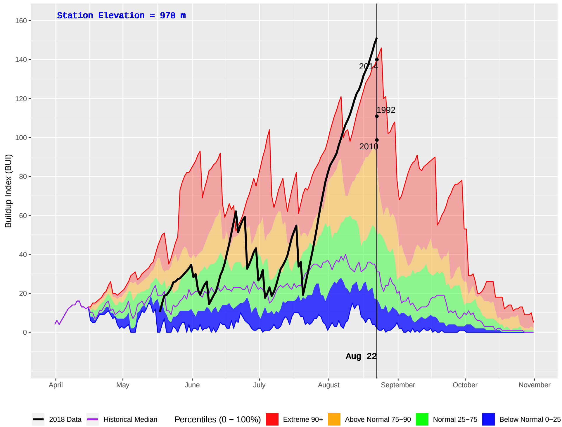
NILKITKWA (172) : Historical (1986–2016) and Current (2018) Daily Buildup Index (BUI)
