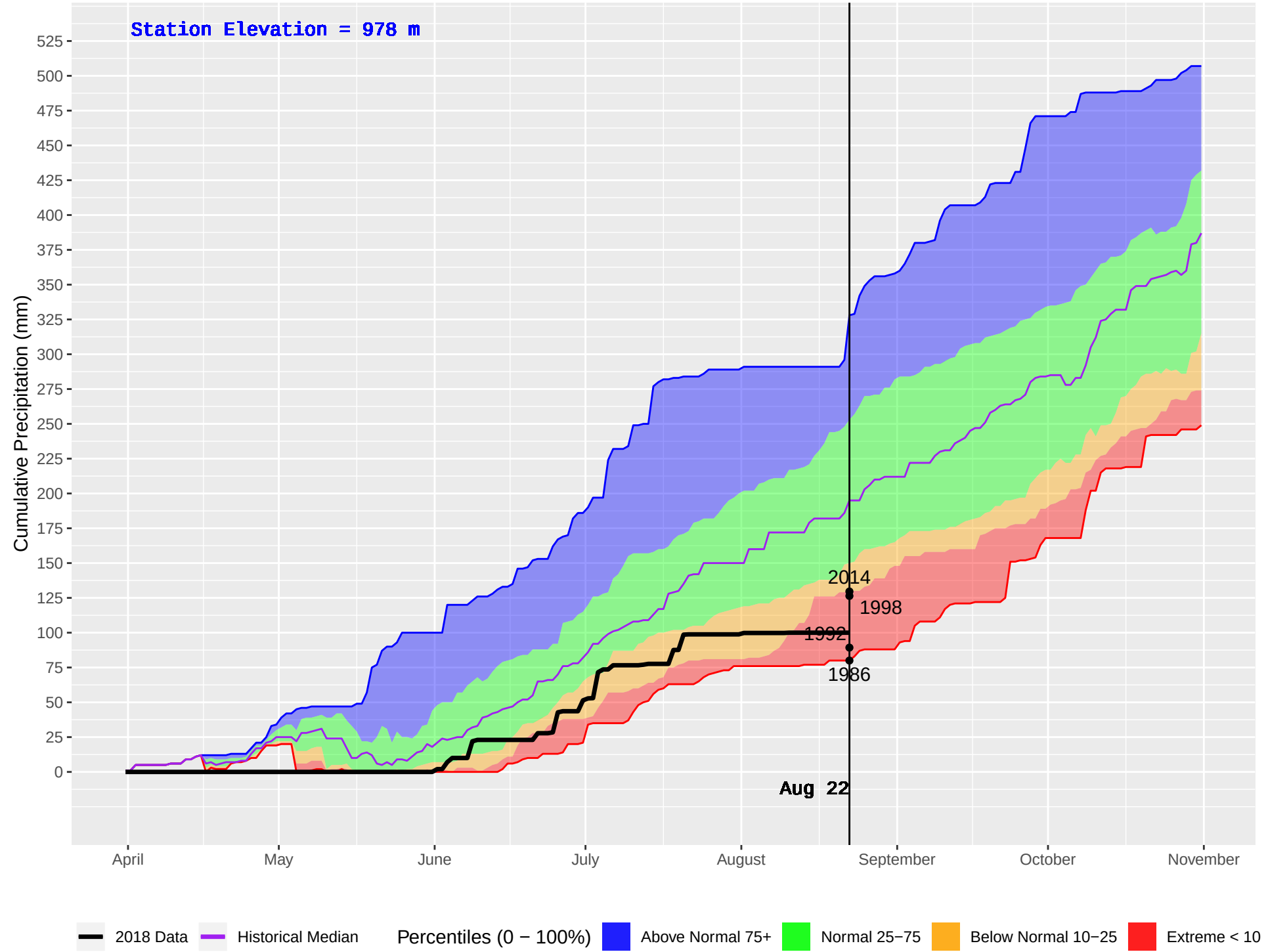
NILKITKWA (172) : Historical (1986–2016) and Current (2018) Daily Cumulative Precipitation
