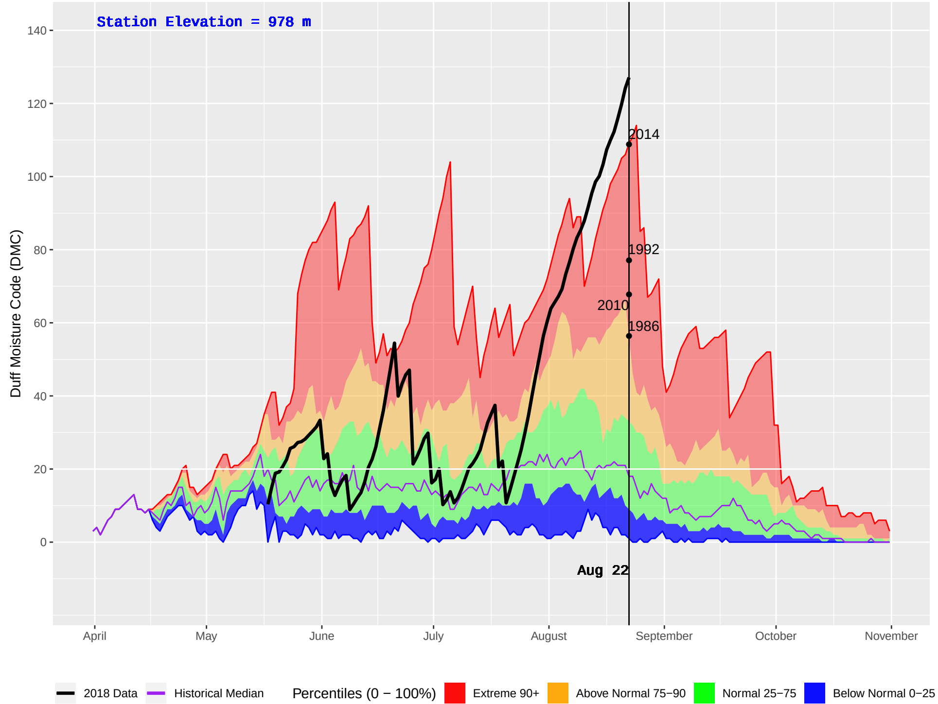
NILKITKWA (172) : Historical (1986–2016) and Current (2018) Daily Duff Moisture Code (DMC)
