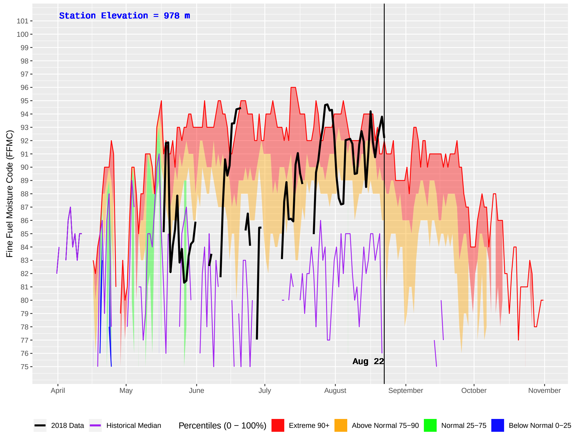
NILKITKWA (172) : Historical (1986–2016) and Current (2018) Daily Fine Fuel Moisture Code (FFMC)
